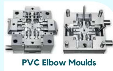
PVC Moulds
